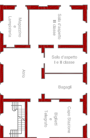
PIANO TERRA
